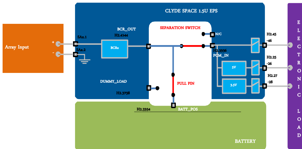
Figure 12-4 Test set-up with Pull Pin Removed
