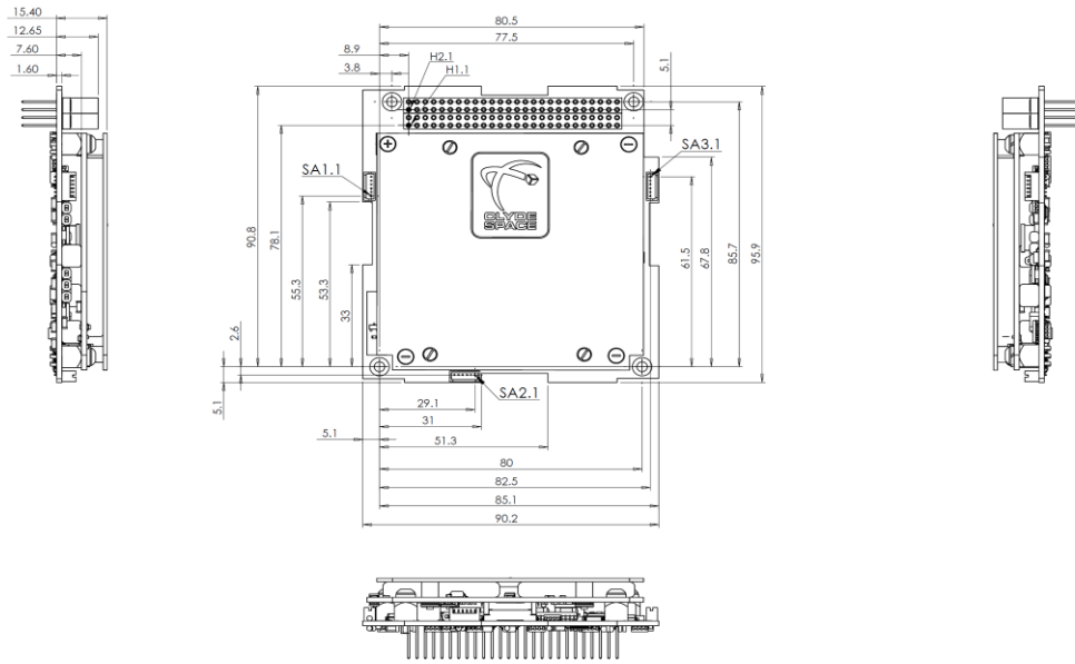
Figure 7-3 1.5U EPS board dimensions (inches)
