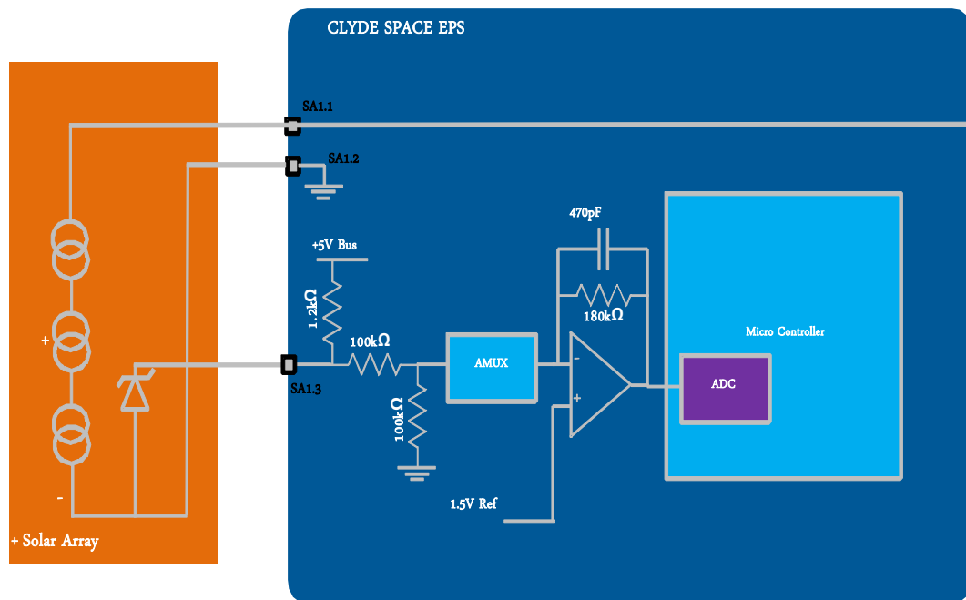
Figure 8-4 Temperature sensor block diagram
