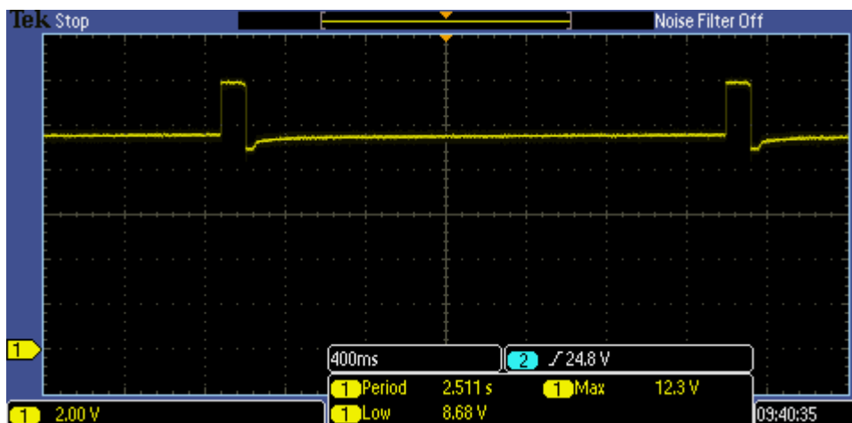
Figure 12-6 Waveform of Solar Array Input
