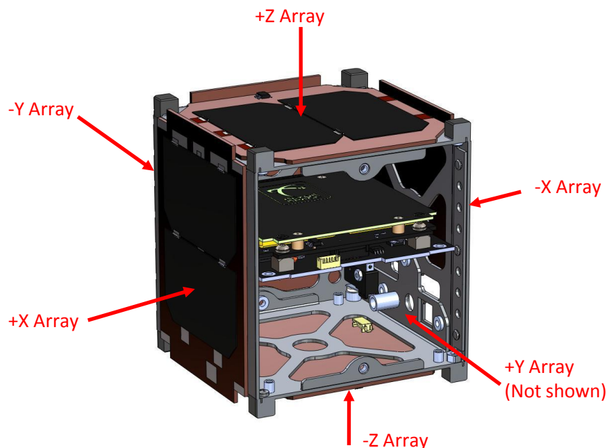
Figure 7-1 Example Array configuration on a 1U EPS.
