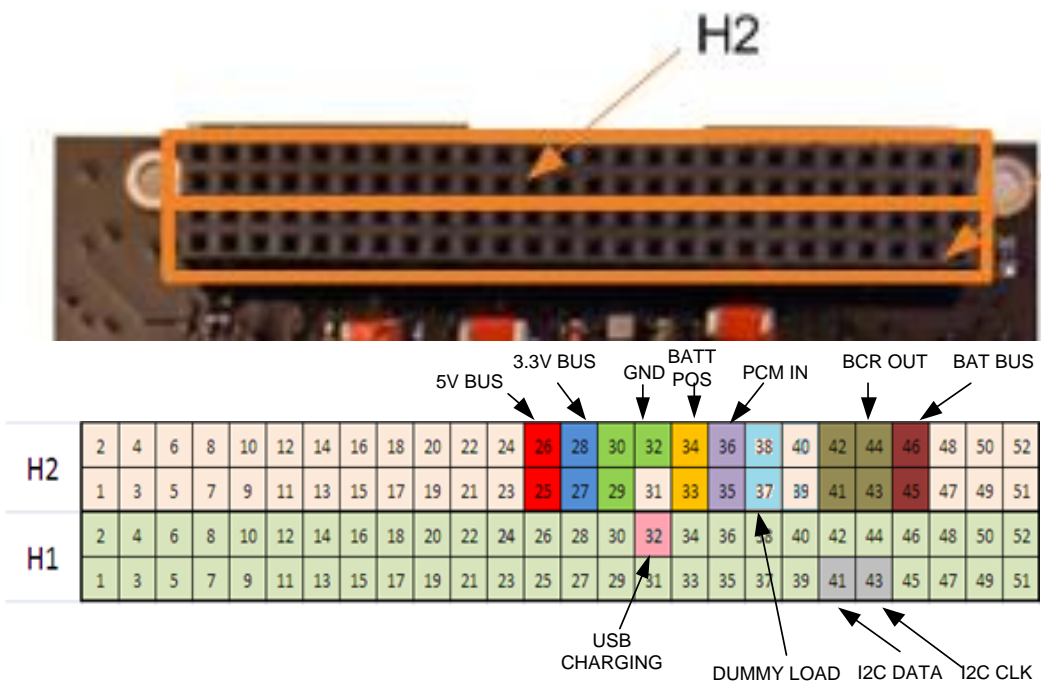
Figure 8-6 EPS Connector Pin Identification
