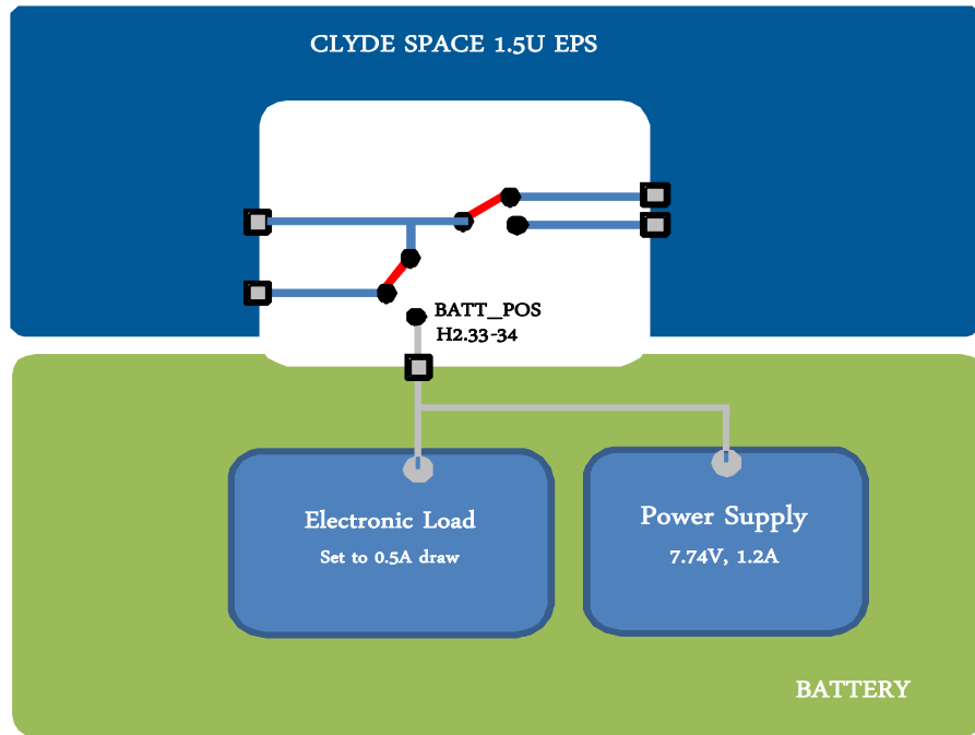
Figure 12-3 Simulated Battery Setup
