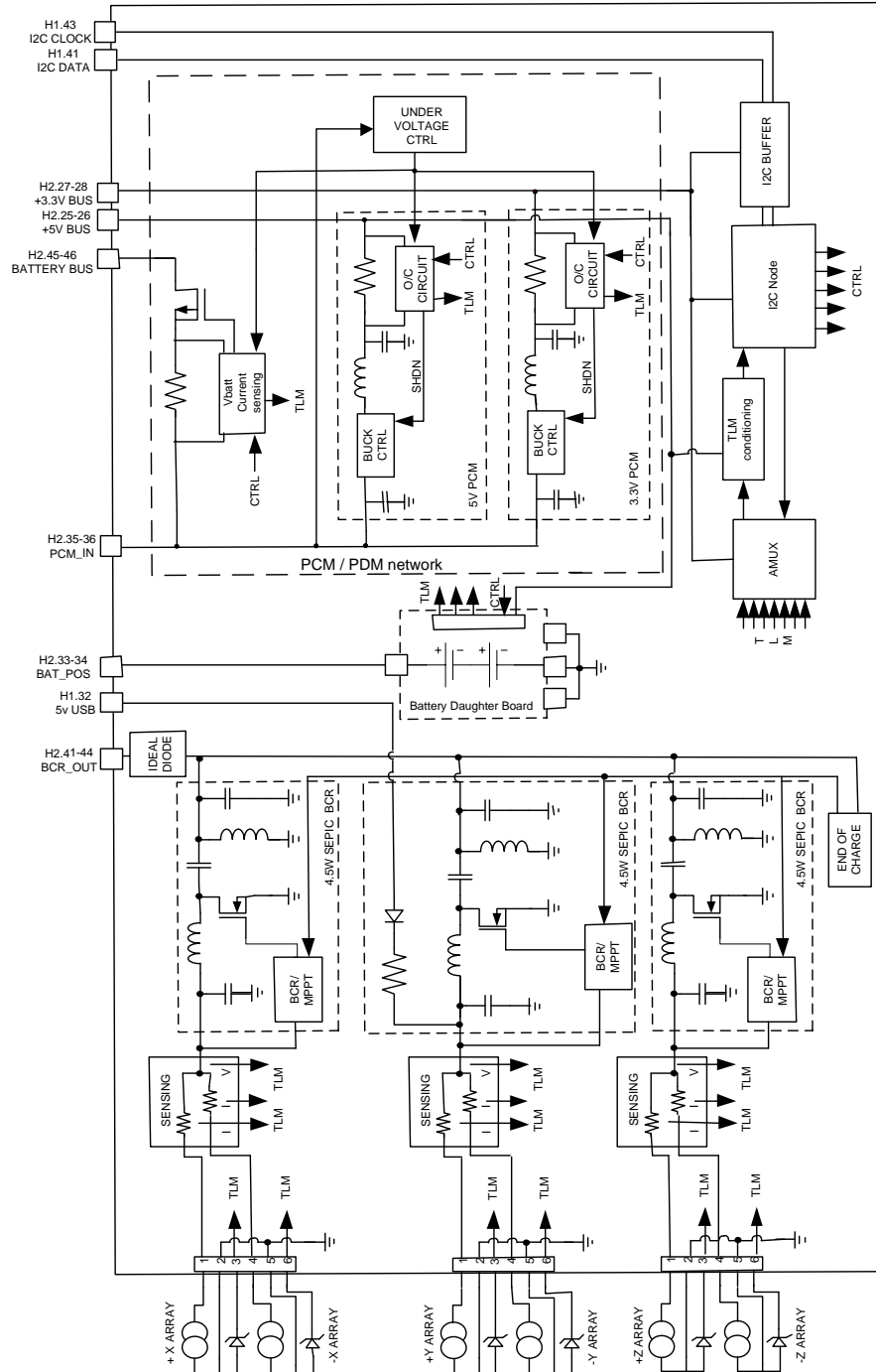
Figure 7-2 Function Diagram
