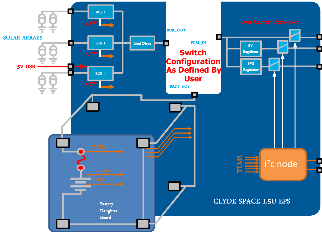
Figure 1-1 System Diagram
