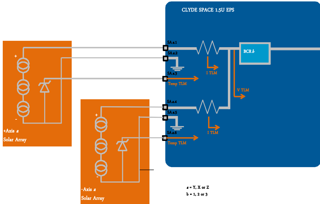
Figure 8-2 Solar Array Configuration
