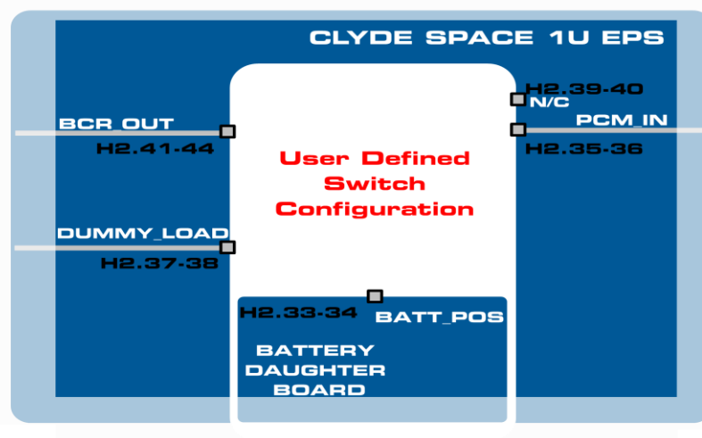
Figure 8-7 Switch connection points
