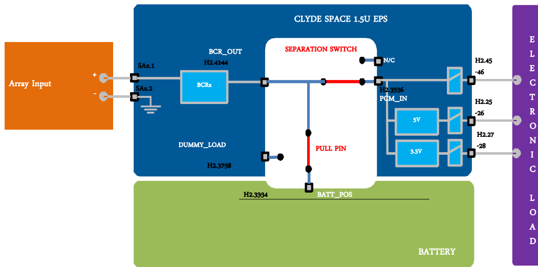
Figure 12-5 Test set-up in Flight Configuration
