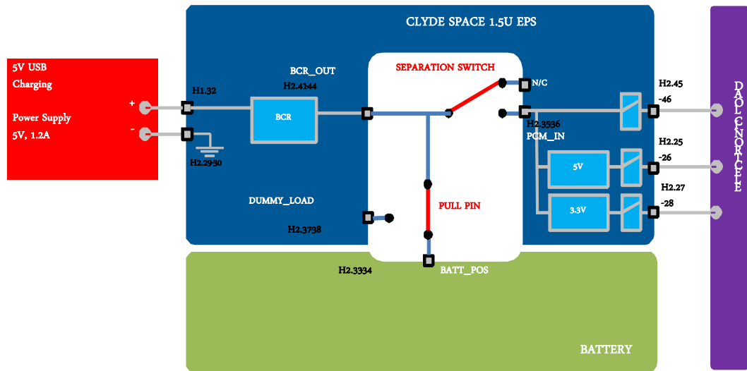
Figure 12-7 USB charge set-up
