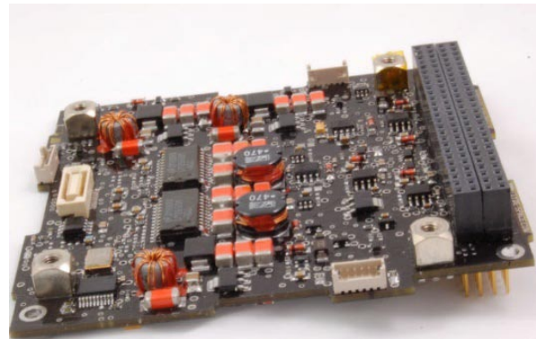
Figure 2 1U CubeSat Power System without battery.
