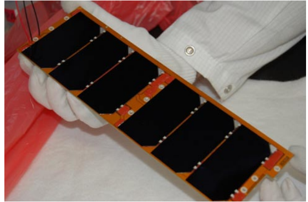
Figure 5 Solar panel for a 3U CubeSat.
