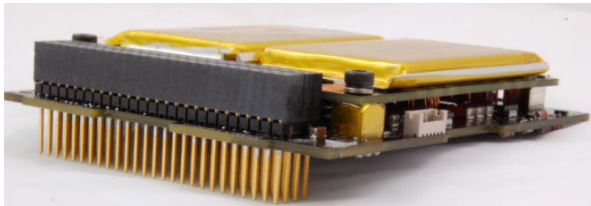
Figure 3 1U CubeSat Power System with battery.
