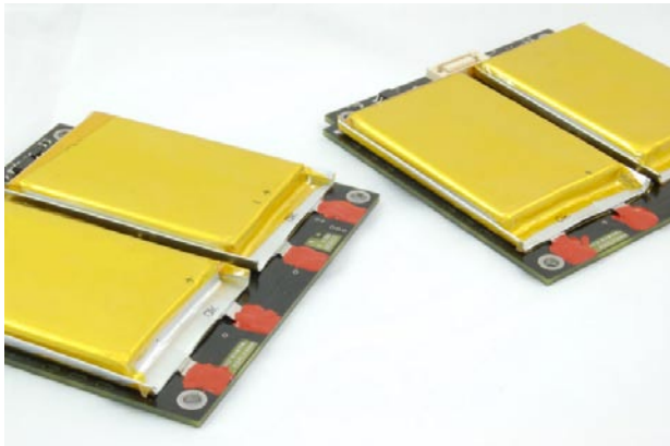
Figure 4 Battery Daughter Boards; 1.25Ah at 8.2V
