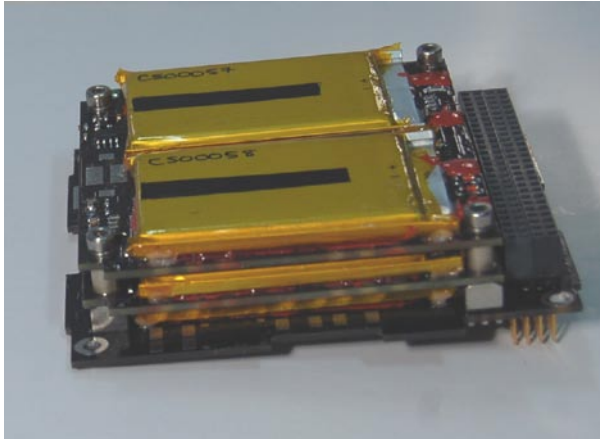
Figure 7 3U/2U 30Whr Battery.
