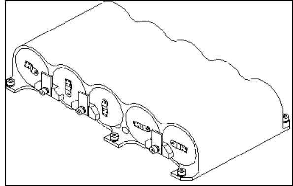
Figure 4.1: Battery Pack of 5 Cells in Series.
