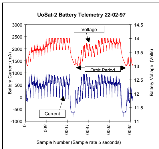
Figure 7.1 - UoSAT-2 Battery Telemetry
