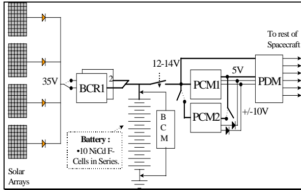
Figure 5.1: Power System Block Diagram
