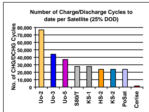
Figure 7.2: Breakdown of Charge/Discharge Cycles
