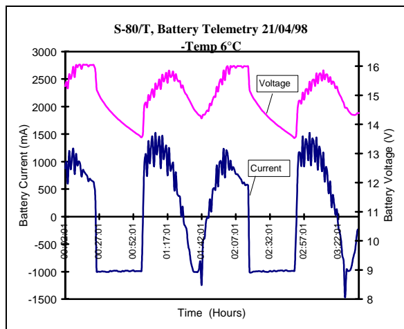
Figure 7.3 In Flight Data from S-80/T
